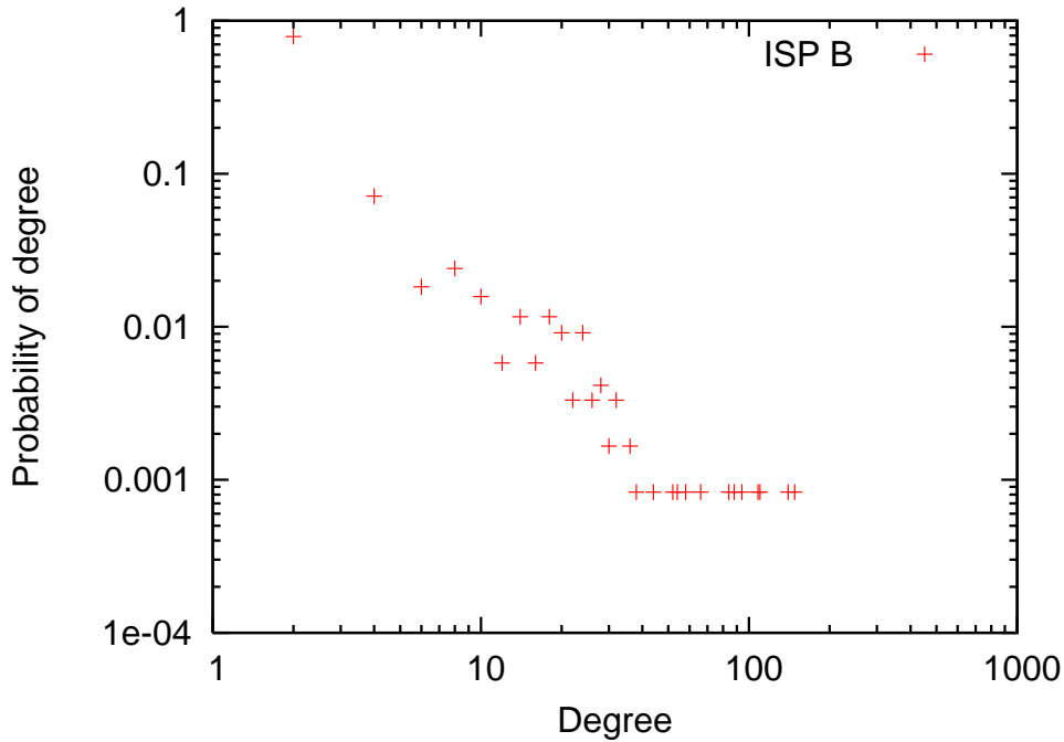
Figure 6: Degree distributions: ISP B
