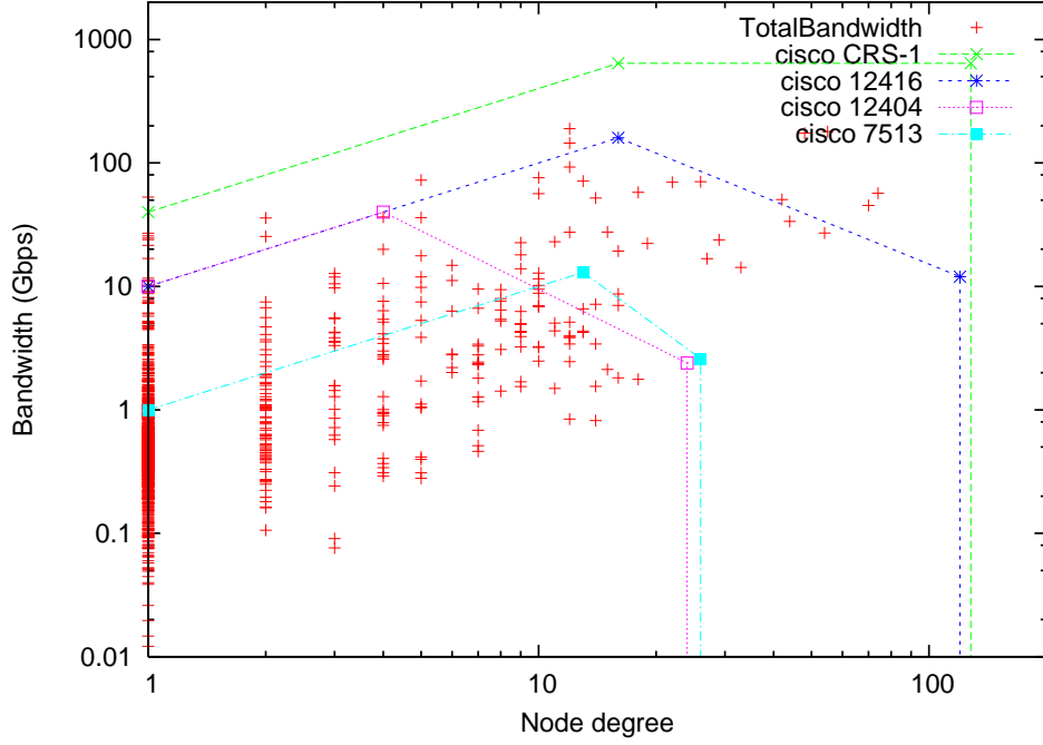
Figure 5: Distributions of totalbandwidth: ISP B
