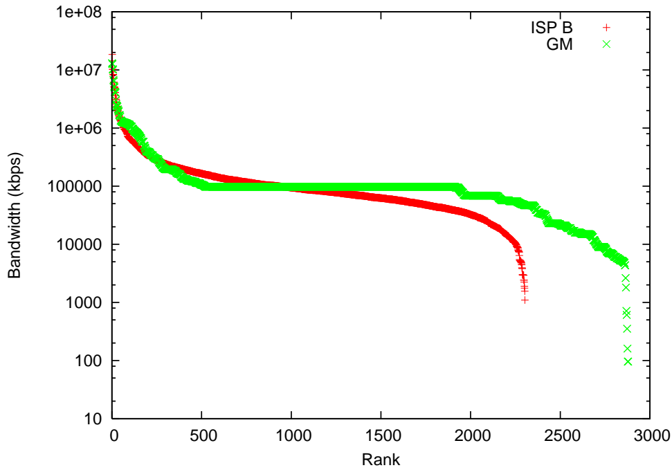
Figure 7: measurement bandwidth and models
