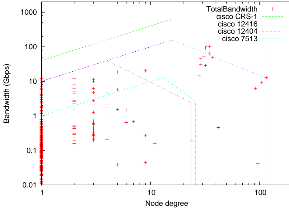
Figure 4: Distributions of totalbandwidths: ISP A
