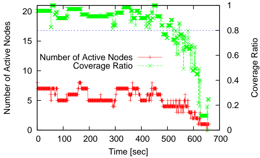
(b) Phase control method with sleep control.
