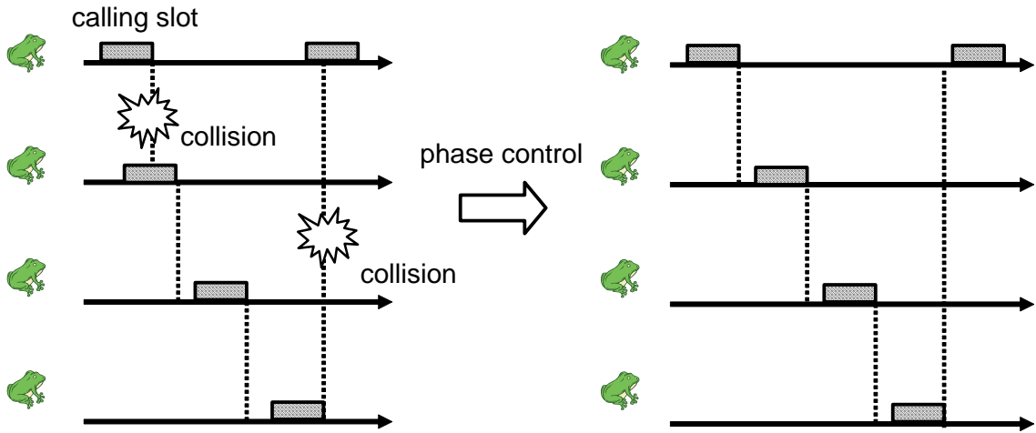
Figure 4: Outline of phase control which reduces the transmission failure by adjusting the transmission timing.
