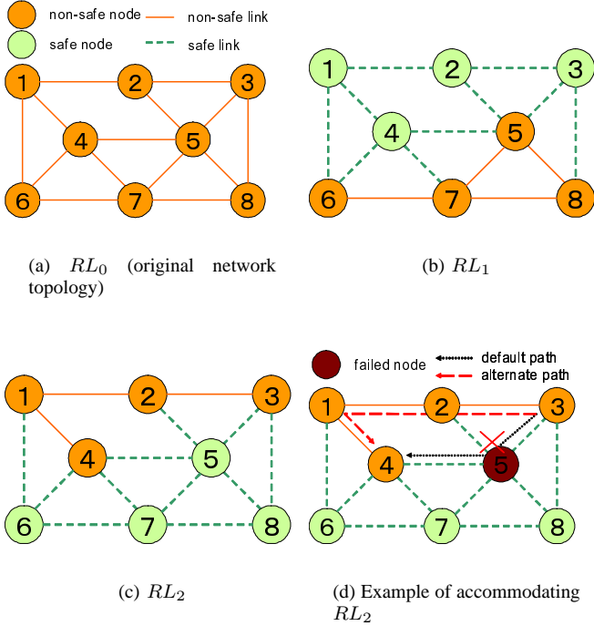
Fig. 1. Example of RLSet. Shown are RL_0 , RL_1 and RL_2
