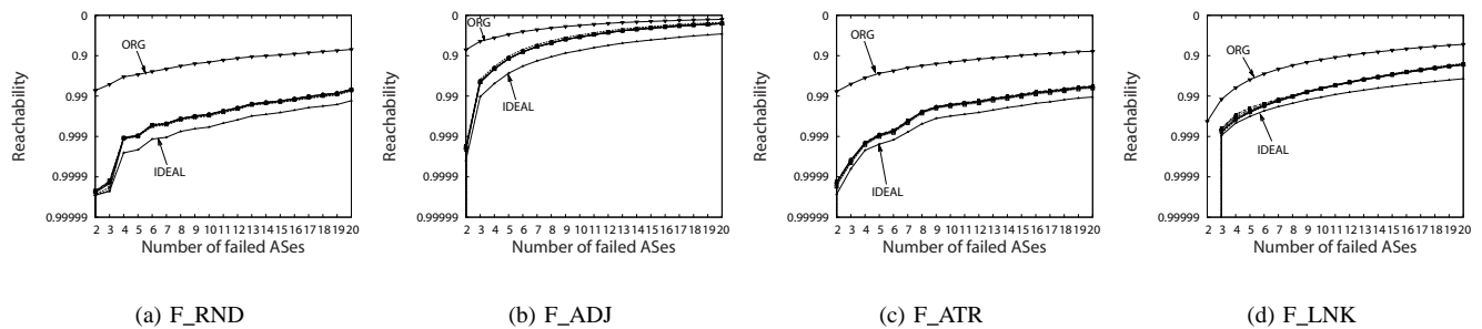
Fig. 6. Network reachability with dynamic RL selection for CASE 2
