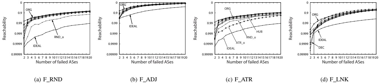
Fig. 4. Network reachability with static RL selection for CASE 1
