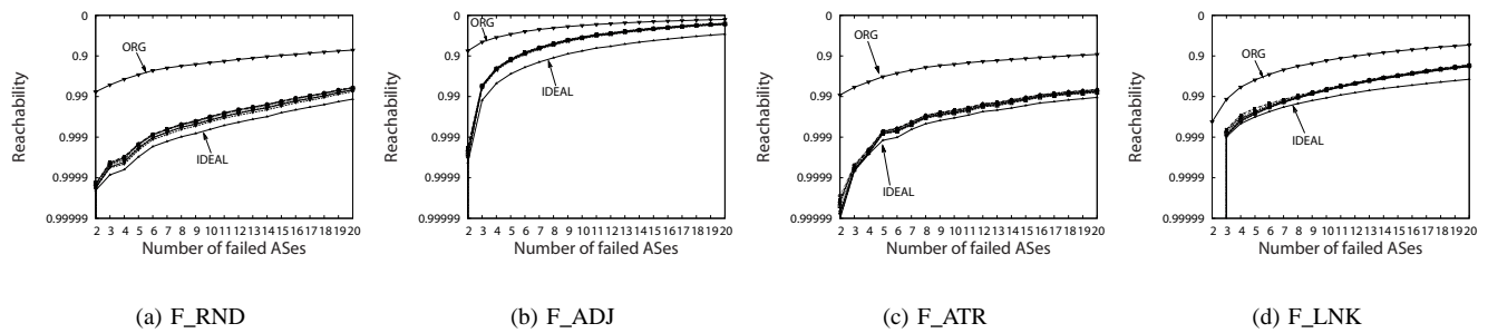
Fig. 5. Network reachability with dynamic RL selection for CASE 1
