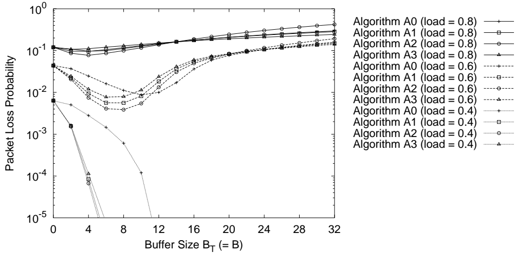
Figure 7. Packet loss probability (shared buffer type switch)
