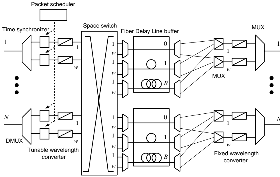
Figure 2. Output buffer type photonic packet switch architecture
