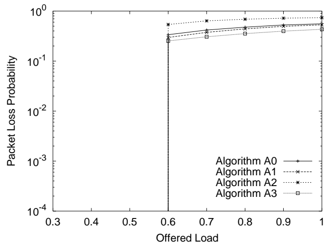
Figure 9. Packet loss probability (shared buffer type switch, for B = 64 )
