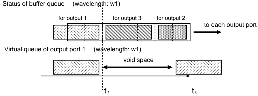
Figure 4. Void space in shared buffer type switch
