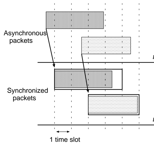
Figure 1. Synchronization of packets inside a switch
