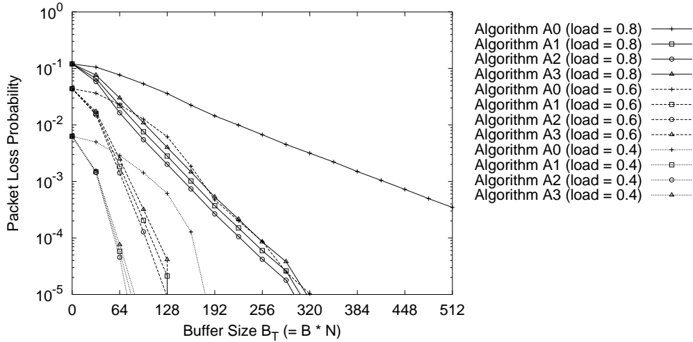
Figure 6. Packet loss probability (output buffer type switch)
