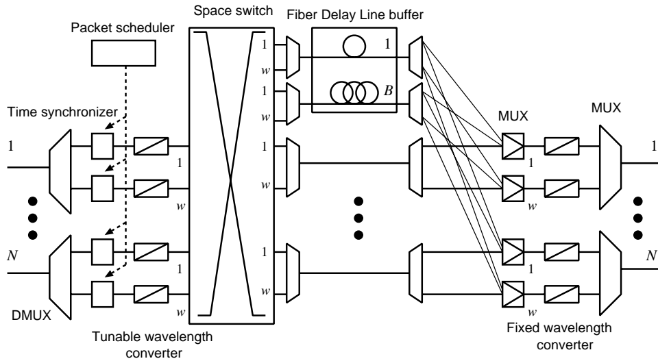
Figure 3. Shared buffer type photonic packet switch architecture
