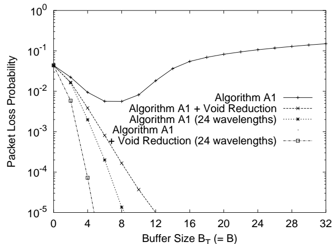
Figure 14. Packet loss probability (shared buffer type switch, void space reduction method + increasing the inner wavelengths, load = 0.6)
