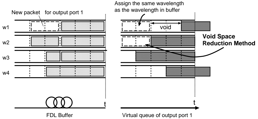
Figure 5. Void space reduction method
