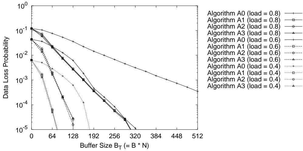
Figure 10. Data loss probability (output buffer type switch)
