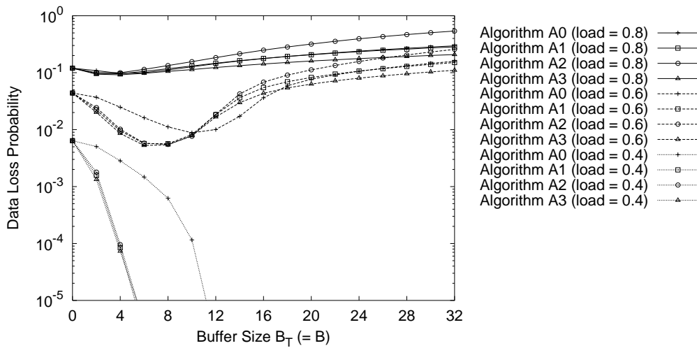
Figure 11. Data loss probability (shared buffer type switch)
