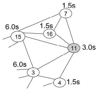
Figure 9. Assignment of an intermittent cycle according to the load for every node
