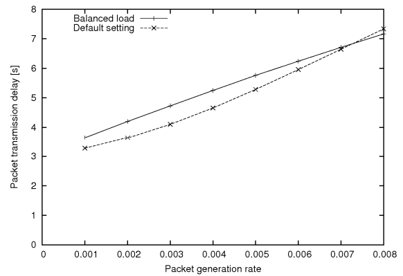
(c) Packet transmission delay
