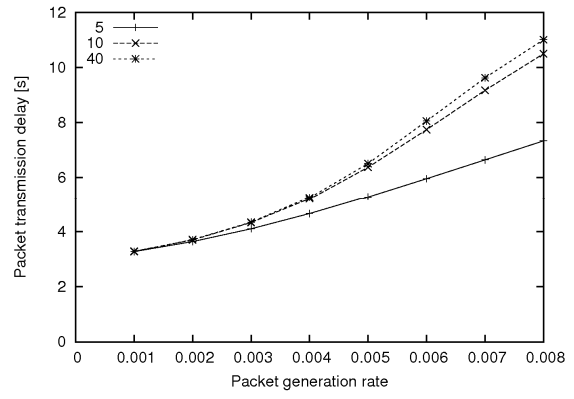
(a) Packet transmission delay
