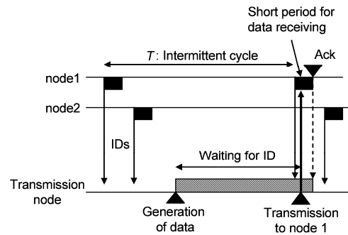
(b) Intermittent Receiver-driven Data Transmission (IRDT)
