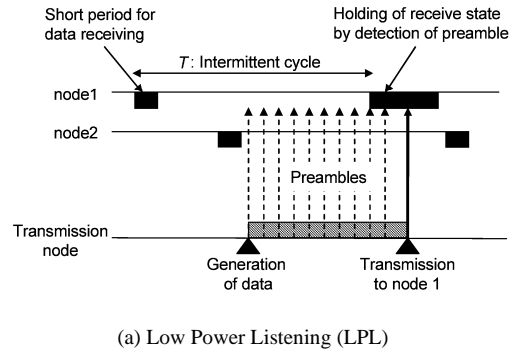
(a) Low Power Listening (LPL)
