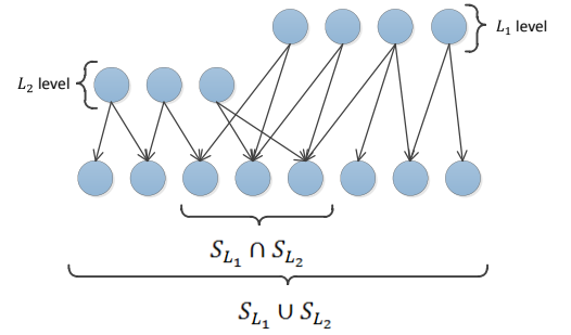
Fig. 6 Modification of definition of degree of collaboration between layers. Here, degree of collaboration between layers is \frac{3}{8} .
