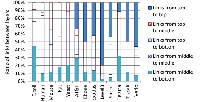
Fig. 3 Ratio of links between each level in hierarchy.
