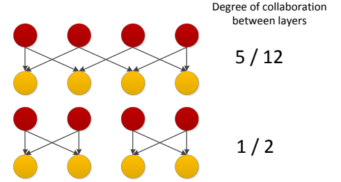
Fig. 5 Illustrative example of how the degree of collaboration between layers defined in [9] differs even when it has the same number of collaboration structure. Both of two topologies (upper and bottom) has the same numbers of nodes / links, and four collaboration structures. In the upper topology, the degree of collaboration between layers is 5/12 , while it is 1/2 in the bottom topology. The difference is caused by the term N_A \cup N_B in Eq. 3. We therefore introduce Eq. 4 such that the degree of collaboration between layers is not affected by the term N_A \cup N_B .
